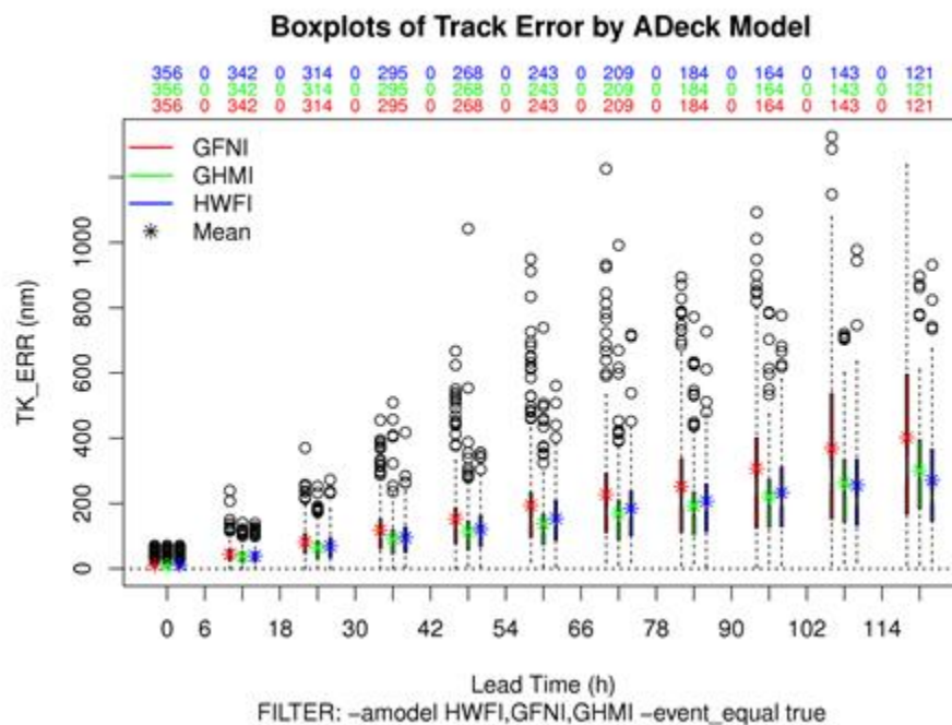
Figure 29.5: Example boxplot from plot_tcmpr.R . Track error distributions by lead time for three operational models GFNI, GHMI, HFWI.
