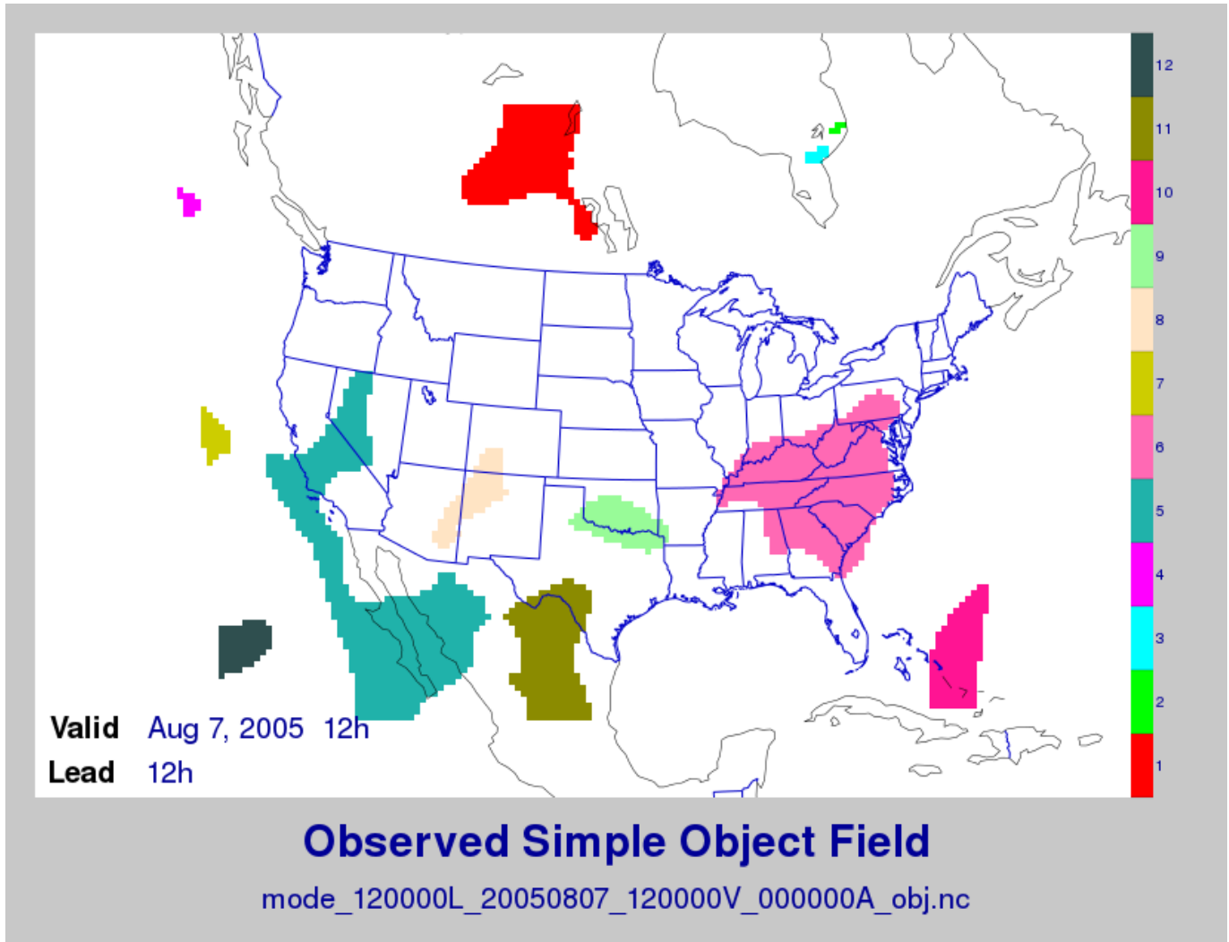
Figure 29.1: Simple observed precipitation objects
