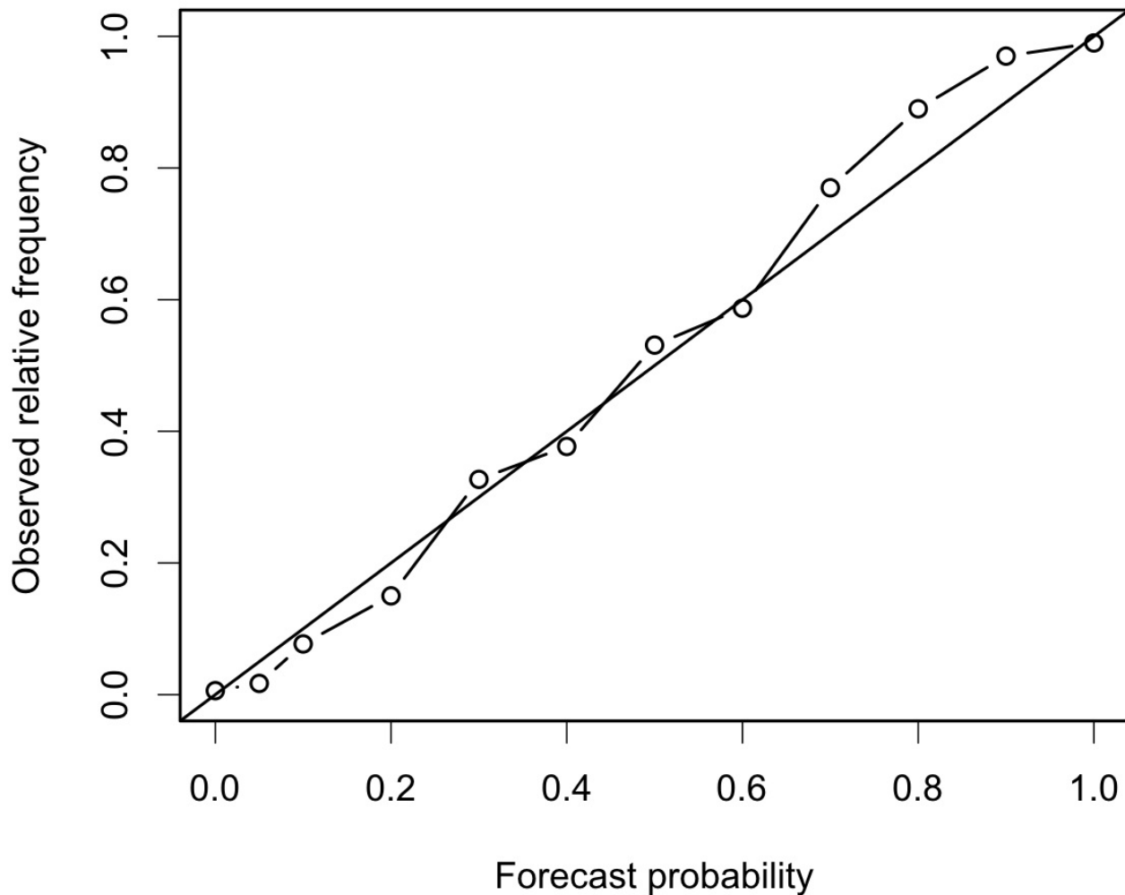
Figure 33.1: Example of Reliability Diagram
