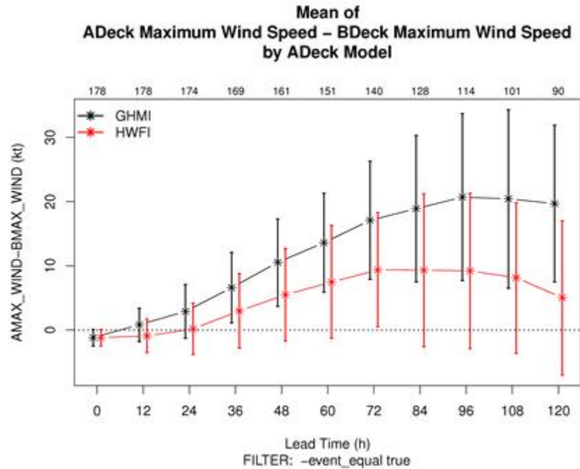
Figure 29.6: Example mean intensity error with confidence intervals at 95% from plot_tcpr.R. Raw intensity error by lead time for a homogeneous comparison of two operational models GHMI, HWFI.
