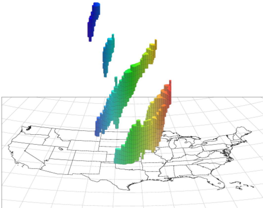
Figure 20.1: MTD Spacetime Objects
