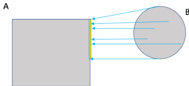
Figure 11.2: Diagram depicting the shortest distances from one event area to another. The yellow bar indicates the part of the event area A to where all of the shortest distances from B are calculated. That is, the shortest distances from every point inside the set B to the set A all point to a point along the yellow bar.
