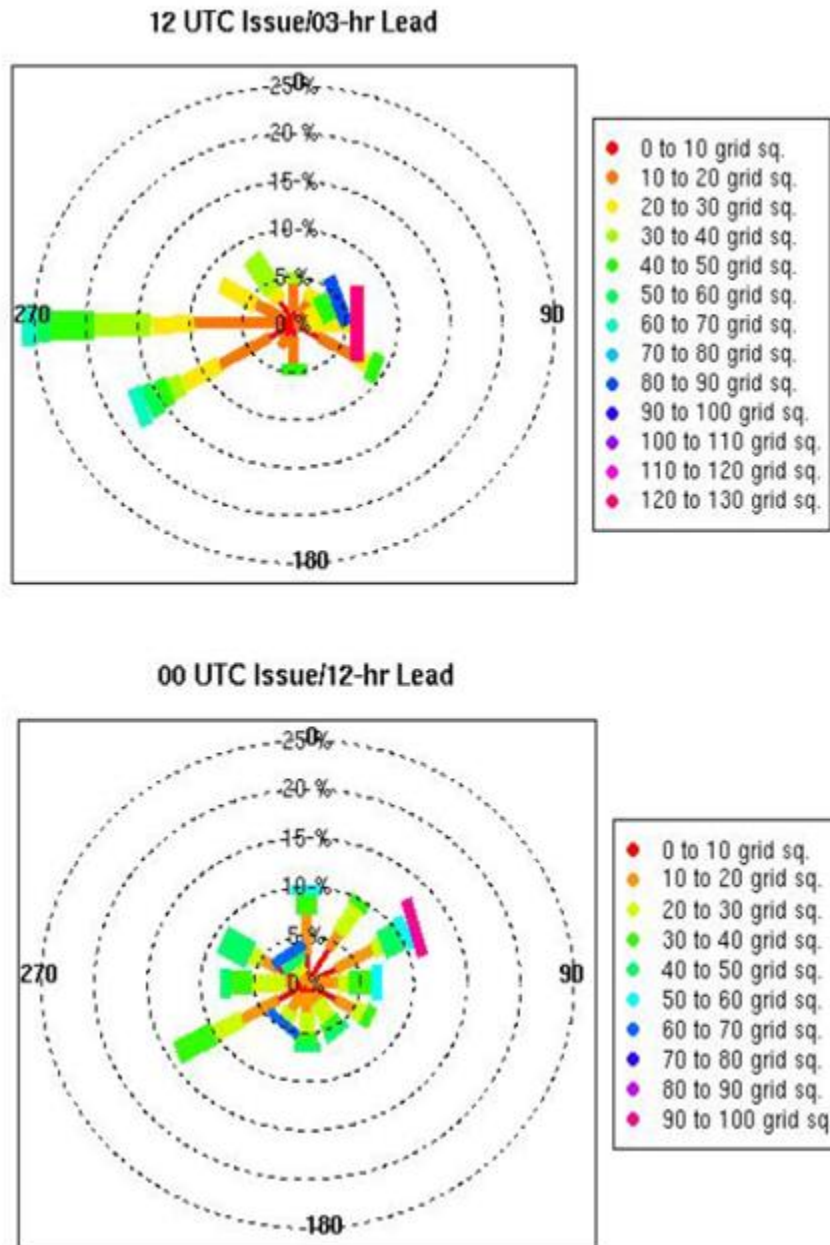
Figure 28.4: Circle histograms showing object centroid angles and distances (see text for explanation).
