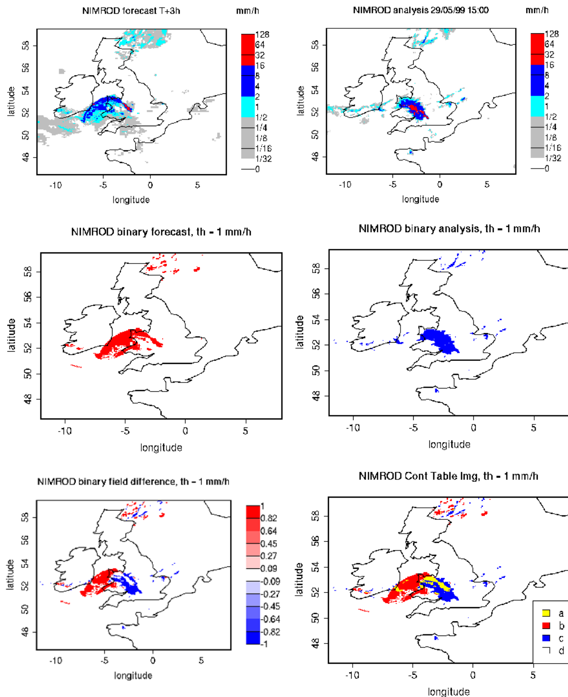
Figure 13.1: NIMROD 3h lead-time forecast and corresponding verifying analysis field (precipitation rate in mm/h, valid the 05/29/99 at 15:00 UTC); forecast and analysis binary fields obtained for a threshold of 1mm/h, the binary field difference has their corresponding Contingency Table Image (see Table 13.1 ). The forecast shows a storm of 160 km displaced almost its entire length.
