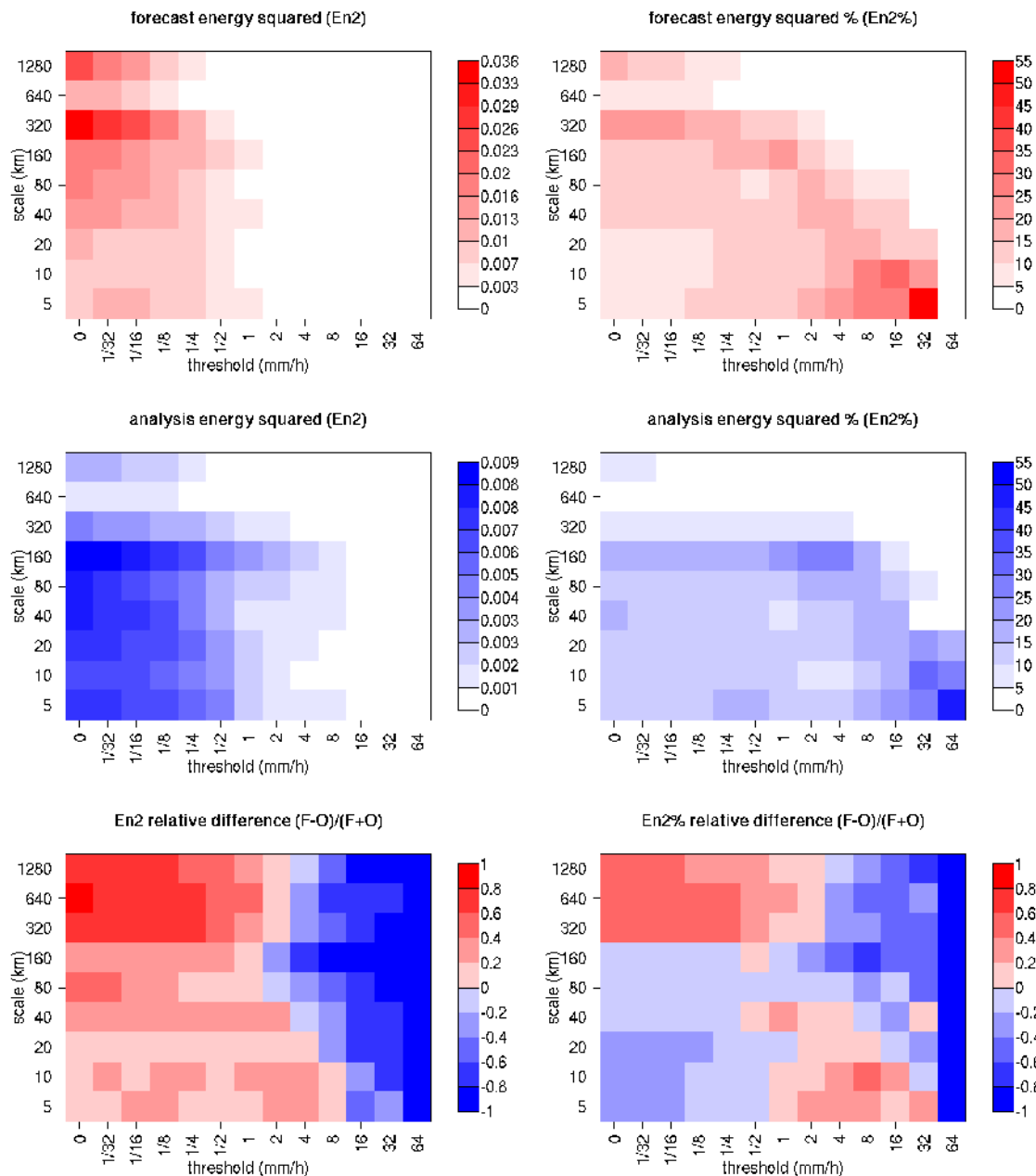
Figure 13.6: Energy squared and energy squared percentages, for each threshold and sale, for the NIMROD forecast and analysis, and forecast and analysis En2 and En2% relative differences.
