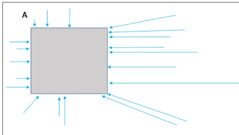
Figure 11.1: The above diagram depicts how a distance map is formed. From every grid point in the domain (depicted by the larger rectangle), the shortest distance from that grid to the nearest non-zero grid point (event; depicted by the gray rectangle labeled as A ) is calculated (a sample of grid points with arrows indicate the path of the shortest distance with the length of the arrow equal to this distance). In a distance map, the value at each grid point is this distance. For example, grid points within the rectangle A will all have value zero in the distance map.
