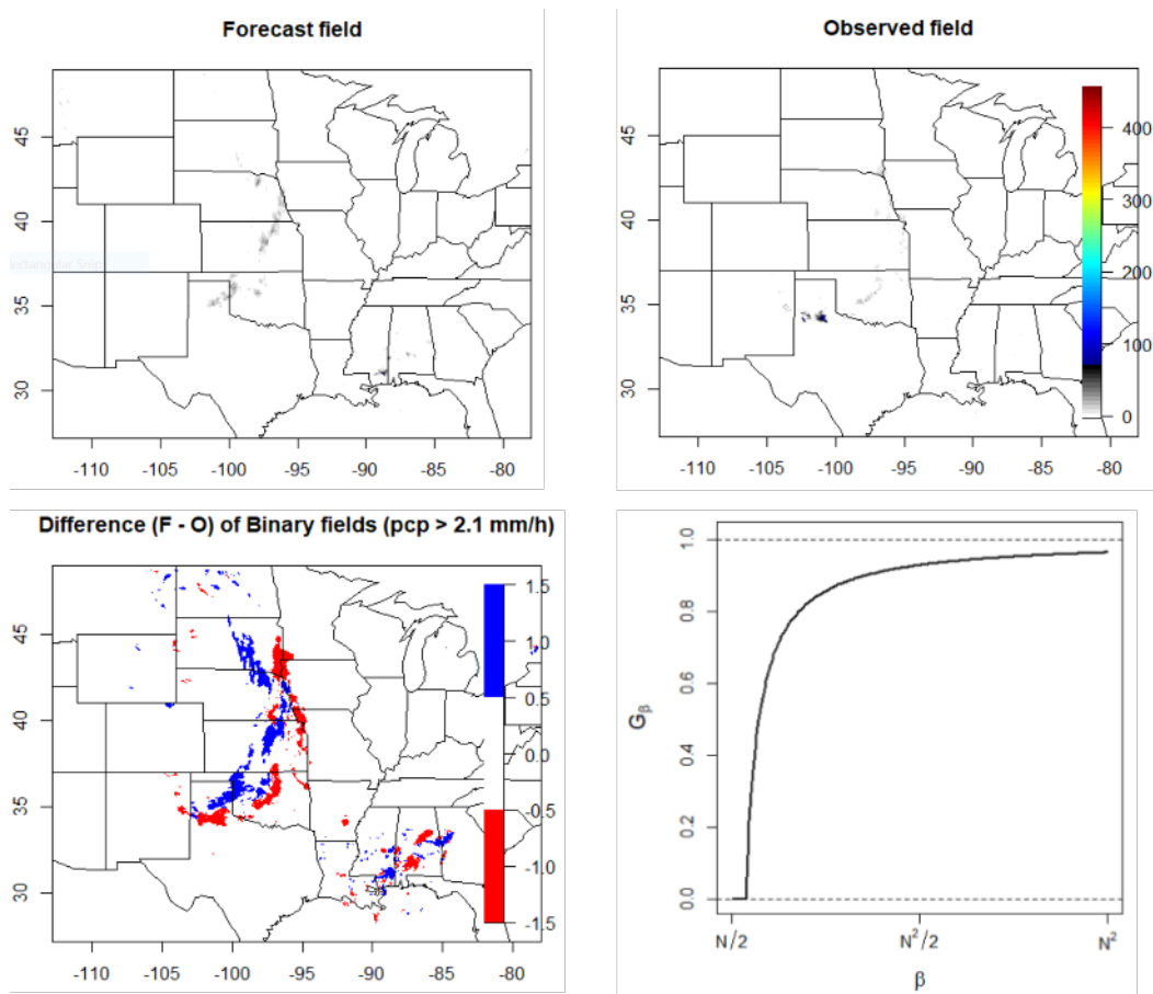
Figure 11.5: Top left is an example of an accumulated precipitation (mm/h) forecast with the corresponding observed field on the top right. Bottom left shows the difference in binary fields, where the binary fields are created by setting all values in the original fields that fall above 2.1\text{mmh}^{-1} to one and the rest to zero. Bottom right shows the results for G_\beta calculated on the binary fields using the threshold of 2.1\text{mmh}^{-1} over a range of choices for \beta .
