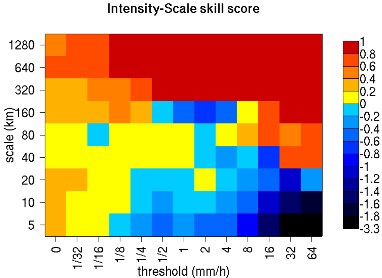
Figure 13.5: Intensity-Scale skill score for the NIMROD forecast and analysis shown in Figure 13.1 . The skill score is a function of the intensity of the precipitation rate and spatial scale of the error. Note the negative skill associated with the scale 6 = 160 km, for the thresholds to 4 mm/h, associated with the displaced storm.
