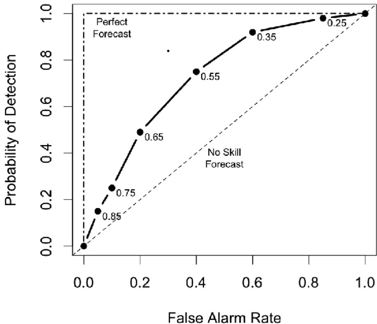
Figure 32.2: Example of ROC Curve
