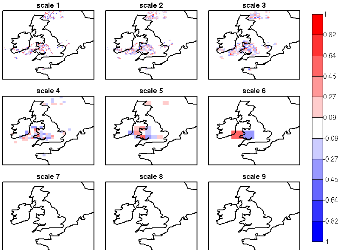
Figure 13.3: NIMROD binary field difference spatial scale components obtained by a 2D Haar wavelet transform ( th=1 mm/h). Scales 1 to 8 refer to mother wavelet components (5, 10, 20, 40, 80, 160, 320, 640 km resolution); scale 9 refers to the largest father wavelet component (1280 km resolution). Note the large error at the scale 6 = 160 km, due to the storm, 160 km displaced almost of its entire length.
