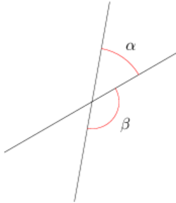
Figure 20.5: Axis Angle Difference
