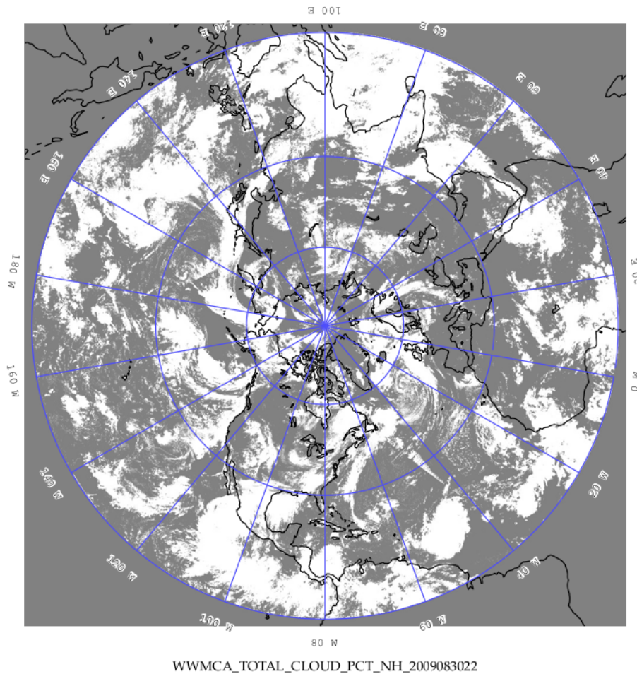
Figure 34.1: Example output of WWMCA-Plot tool.
