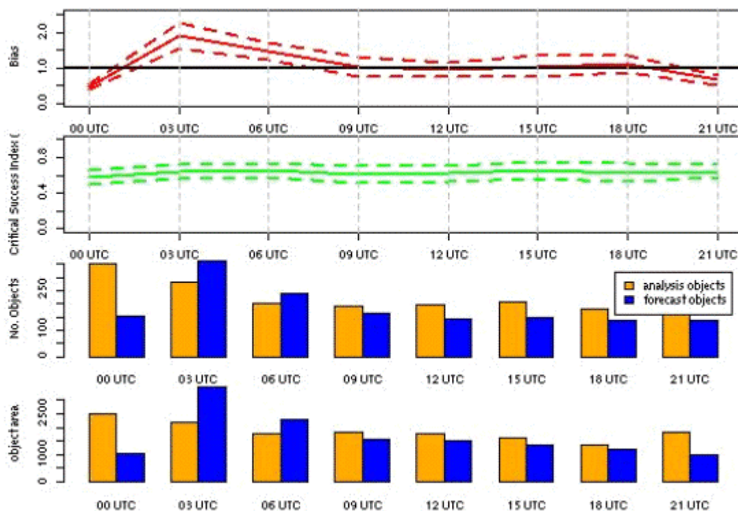
Figure 28.3: Traditional verification scores applied to output of the MODE tool, computed by defining matched observed objects to be hits, unmatched observed objects to be misses, and unmatched forecast objects to be false alarms; weighted by object area. Bar plots show numbers (penultimate row) and areas (bottom row) of observed and forecast objects, respectively.
