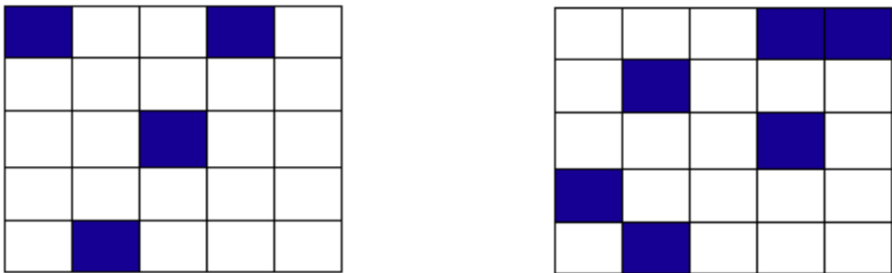
Figure 10.3: Example showing how HiRA proportions are calculated.
