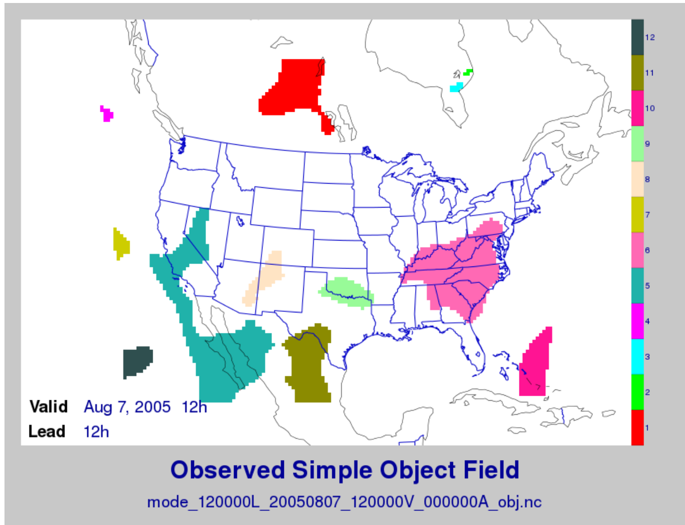
Figure 28.1: Simple observed precipitation objects
