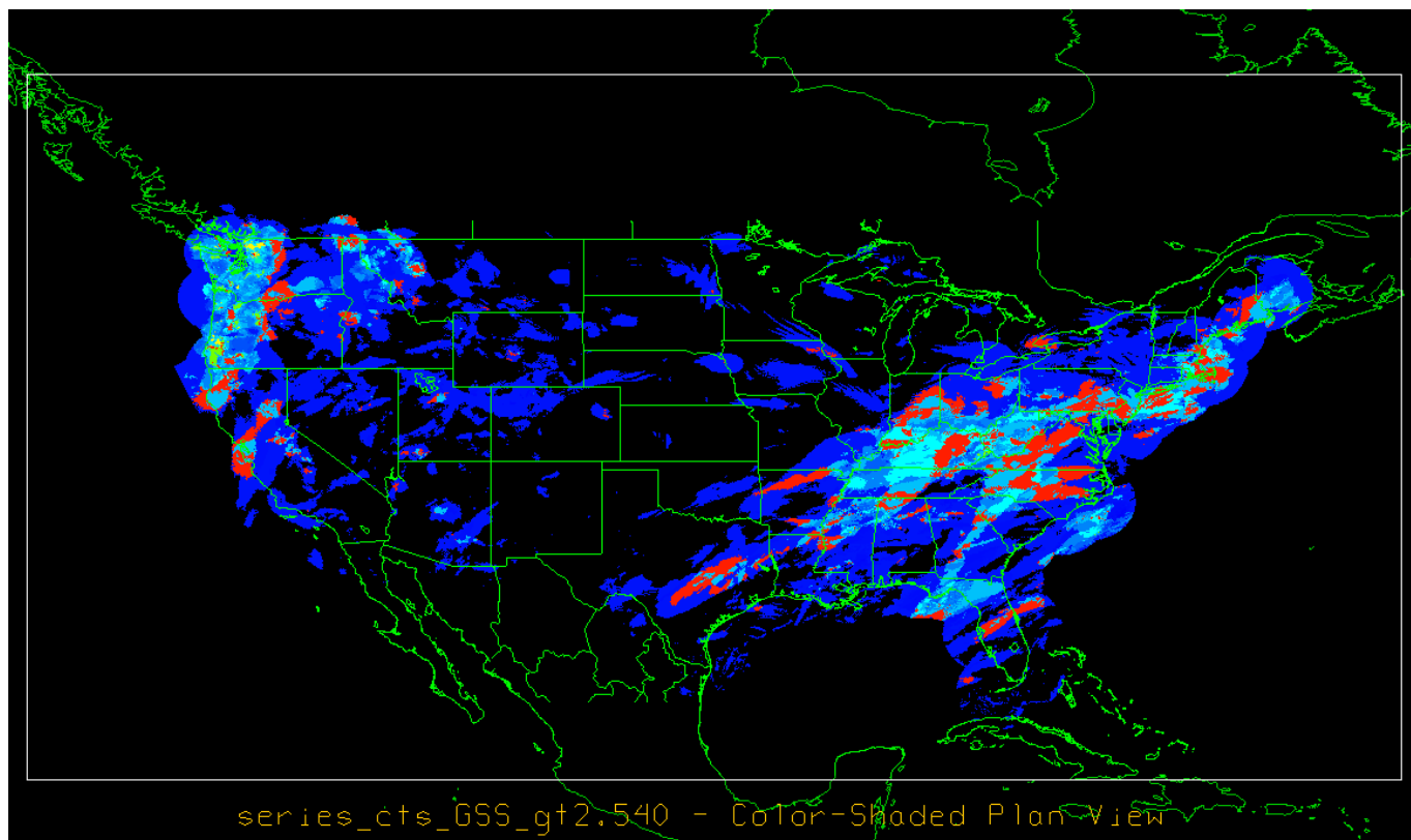
Figure 16.1: An example of the Gilbert Skill Score for precipitation forecasts at each grid location for a month of files.
