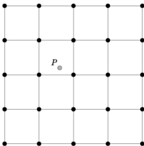
Figure 10.1: Diagram illustrating matching and interpolation methods used in MET. See text for explanation.
