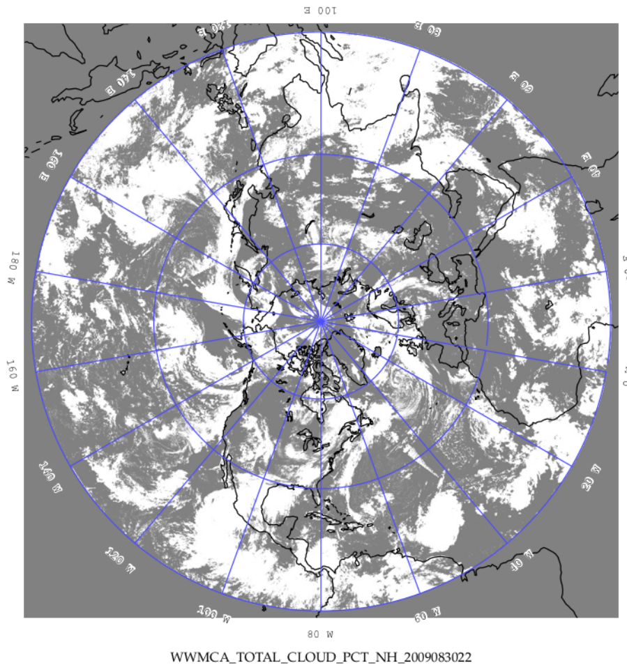
Figure 7.2: Example output of WWMCA-Plot tool.
