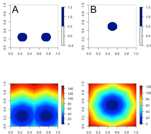
Figure 11.3: Binary fields (top) with event areas A (consisting of two circular event areas) and a second field with event area B (single circular area) with their respective distance maps (bottom).
