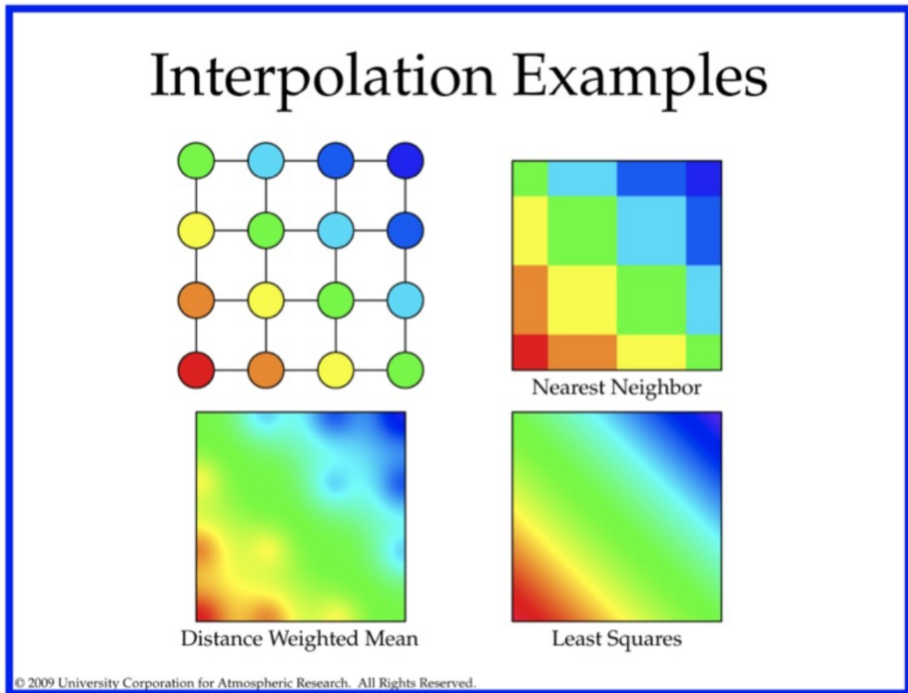
Figure 10.2: Illustration of some matching and interpolation methods used in MET. See text for explanation.
