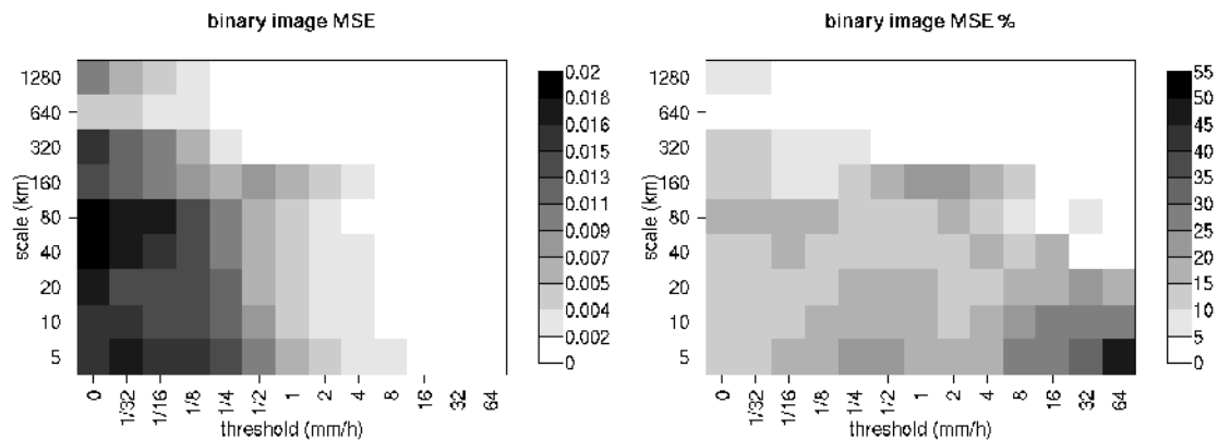
Figure 13.4: MSE and MSE % for the NIMROD binary forecast and analysis spatial scale components. In the MSE%, note the large error associated with the scale 6 = 160 km, for the thresholds \frac{1}{2} to 4 mm/h, associated with the displaced storm.
