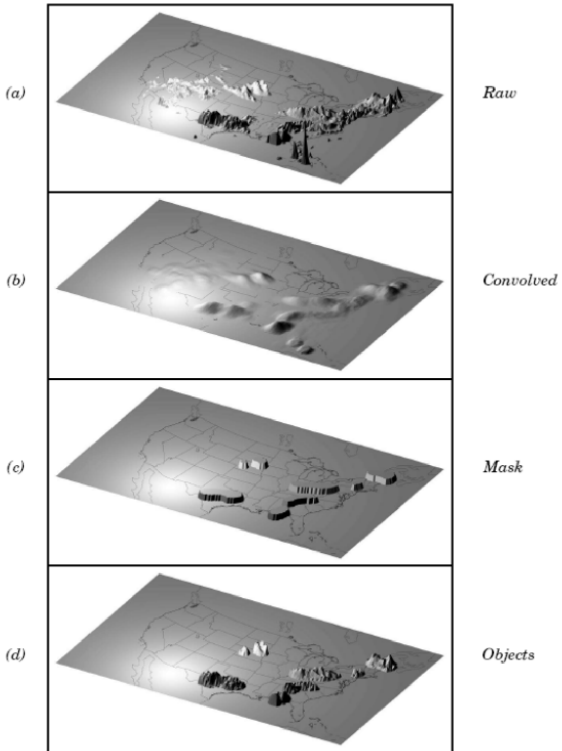
Figure 18.1: Example of an application of the MODE object identification process to a model precipitation field.
