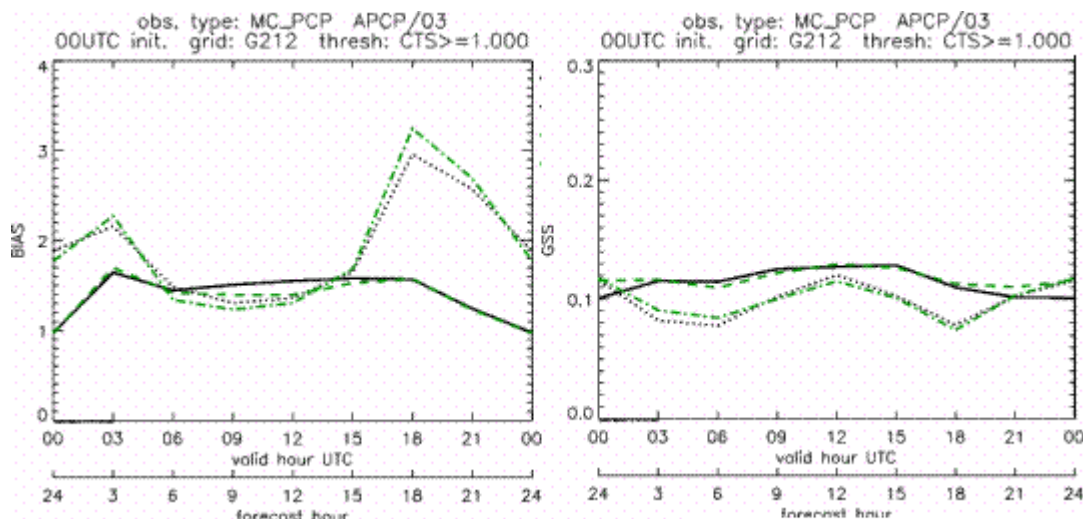
Figure 28.2: Time series of forecast area bias and Gilbert Skill Score for four model configurations (different lines) stratified by time-of-day.
