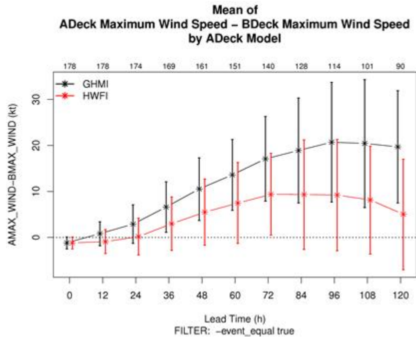
Figure 28.6: Example mean intensity error with confidence intervals at 95% from plot_tcpr.R. Raw intensity error by lead time for a homogeneous comparison of two operational models GHMI, HWFI.
