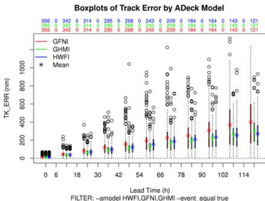
Figure 28.5: Example boxplot from plot_tcmpr.R . Track error distributions by lead time for three operational models GFNI, GHMI, HWFI.
