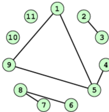
Figure 21.6: Basic Graph Example
