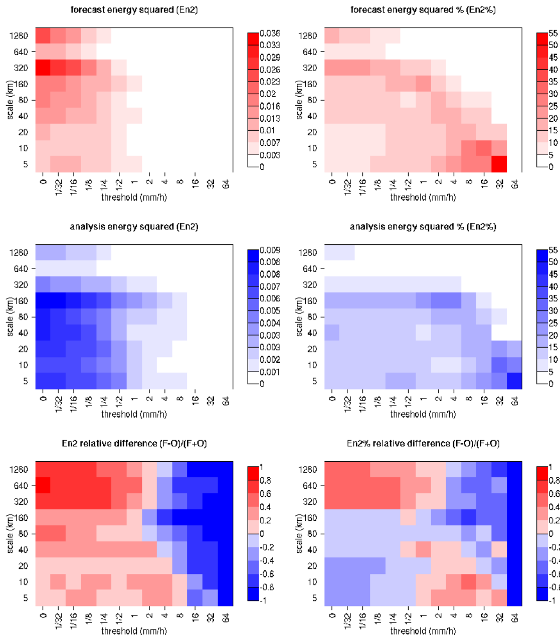
Figure 14.6: Energy squared and energy squared percentages, for each threshold and scale, for the NIMROD forecast and analysis, and forecast and analysis En2 and En2% relative differences.
