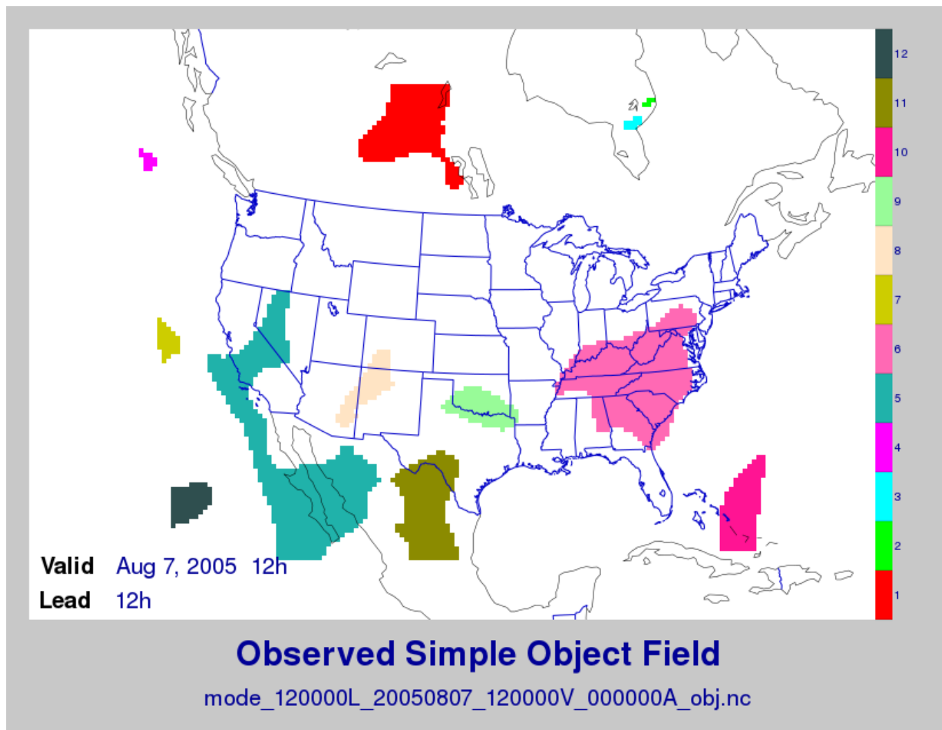
Figure 30.1: Simple observed precipitation objects
