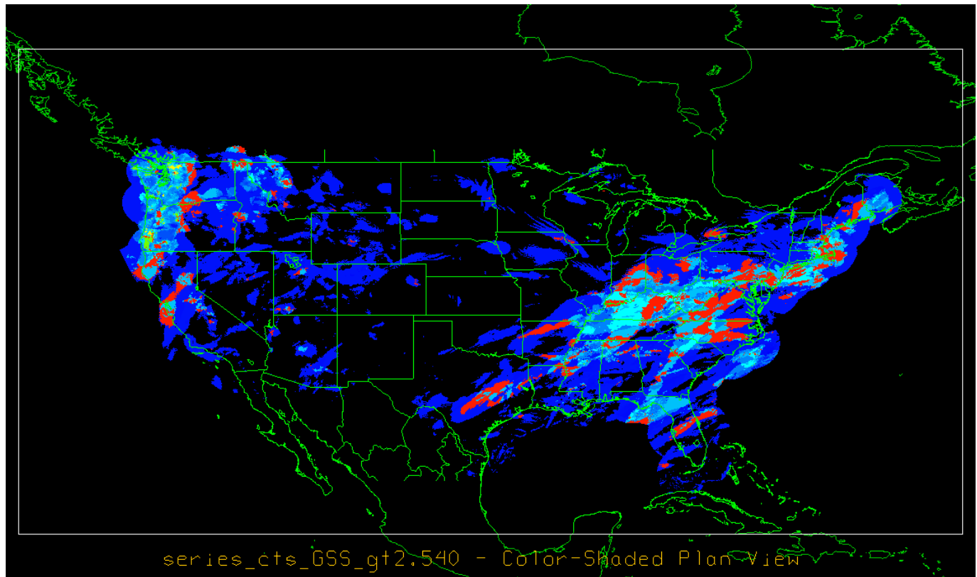
Figure 16.1: An example of the Gilbert Skill Score for precipitation forecasts at each grid location for a month of files.
