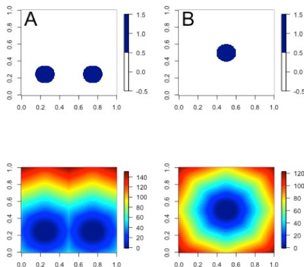
Figure 11.3: Binary fields (top) with event areas A (consisting of two circular event areas) and a second field with event area B (single circular area) with their respective distance maps (bottom).
