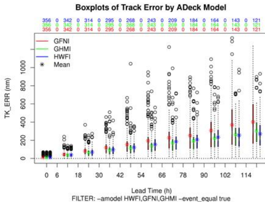
Figure 29.5: Example boxplot from plot_tcmpr.R . Track error distributions by lead time for three operational models GFNI, GHMI, HWFI.
