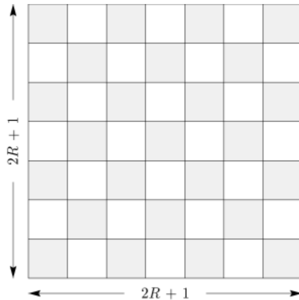
Figure 21.2: Convolution Region
